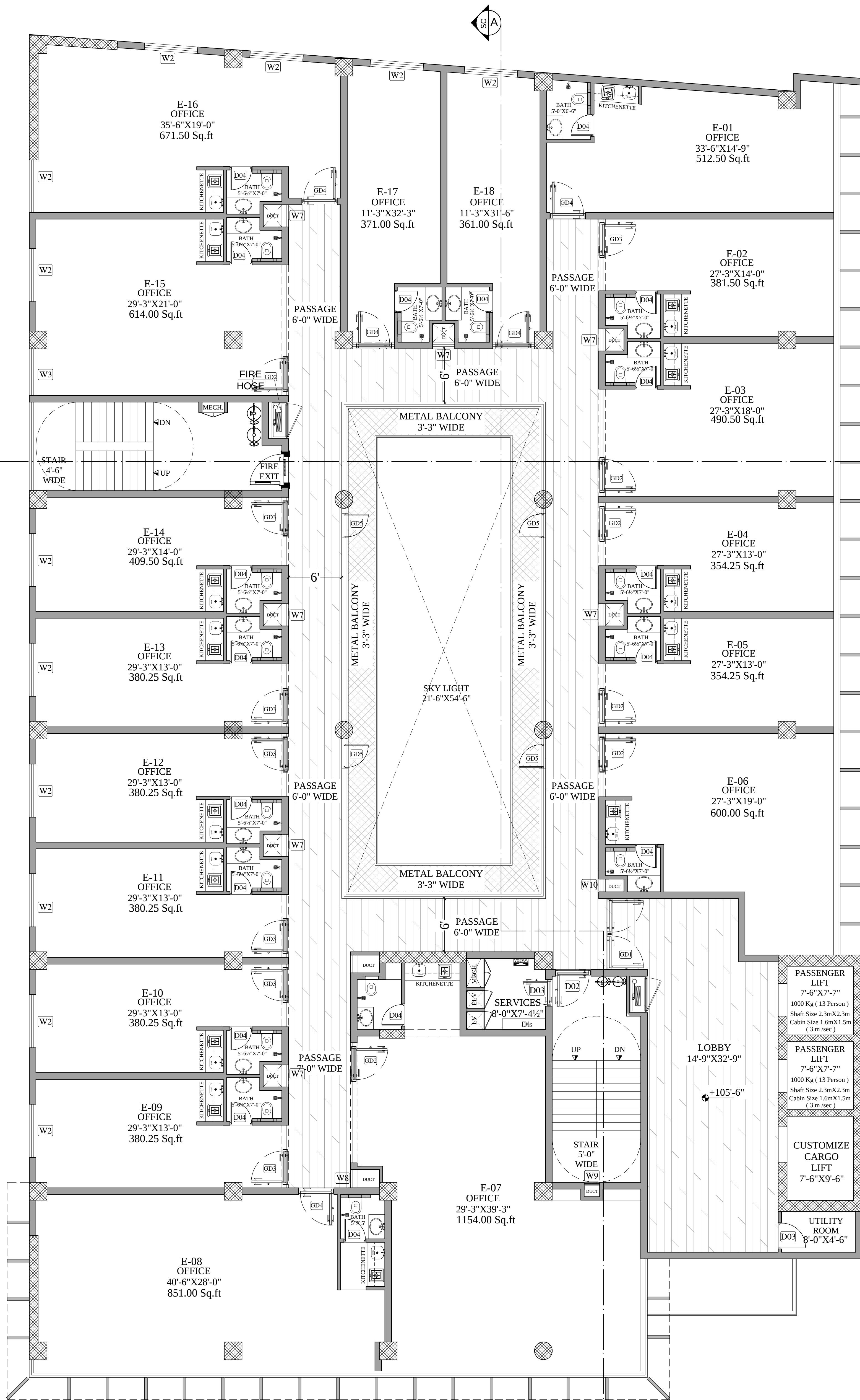
8th FLOOR LAYOUT PLAN COVERED AREA 12058.00 Sq. Ft.
