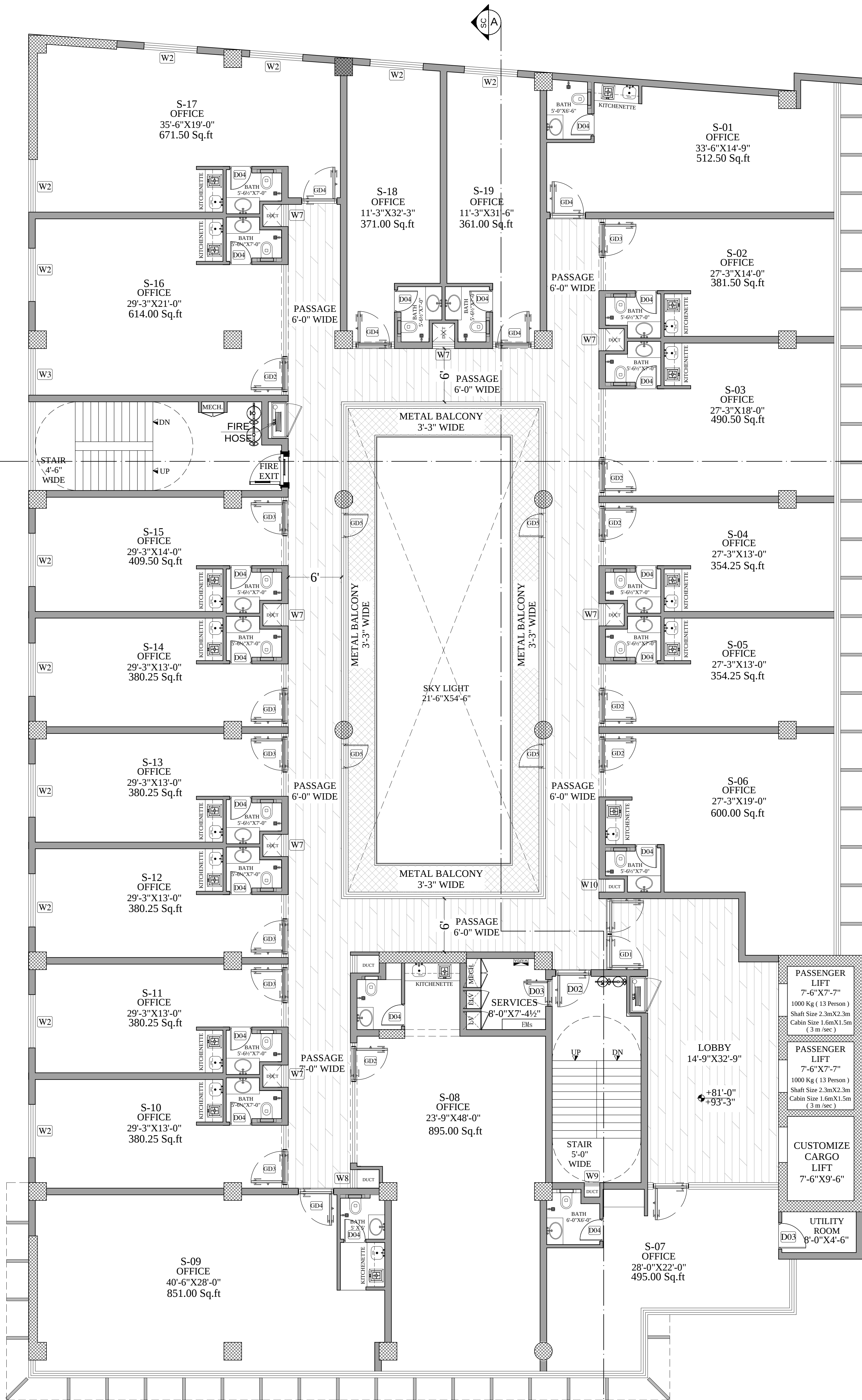
6th & 7th FLOOR LAYOUT PLAN COVERED AREA 12163.00 Sq. Ft.
